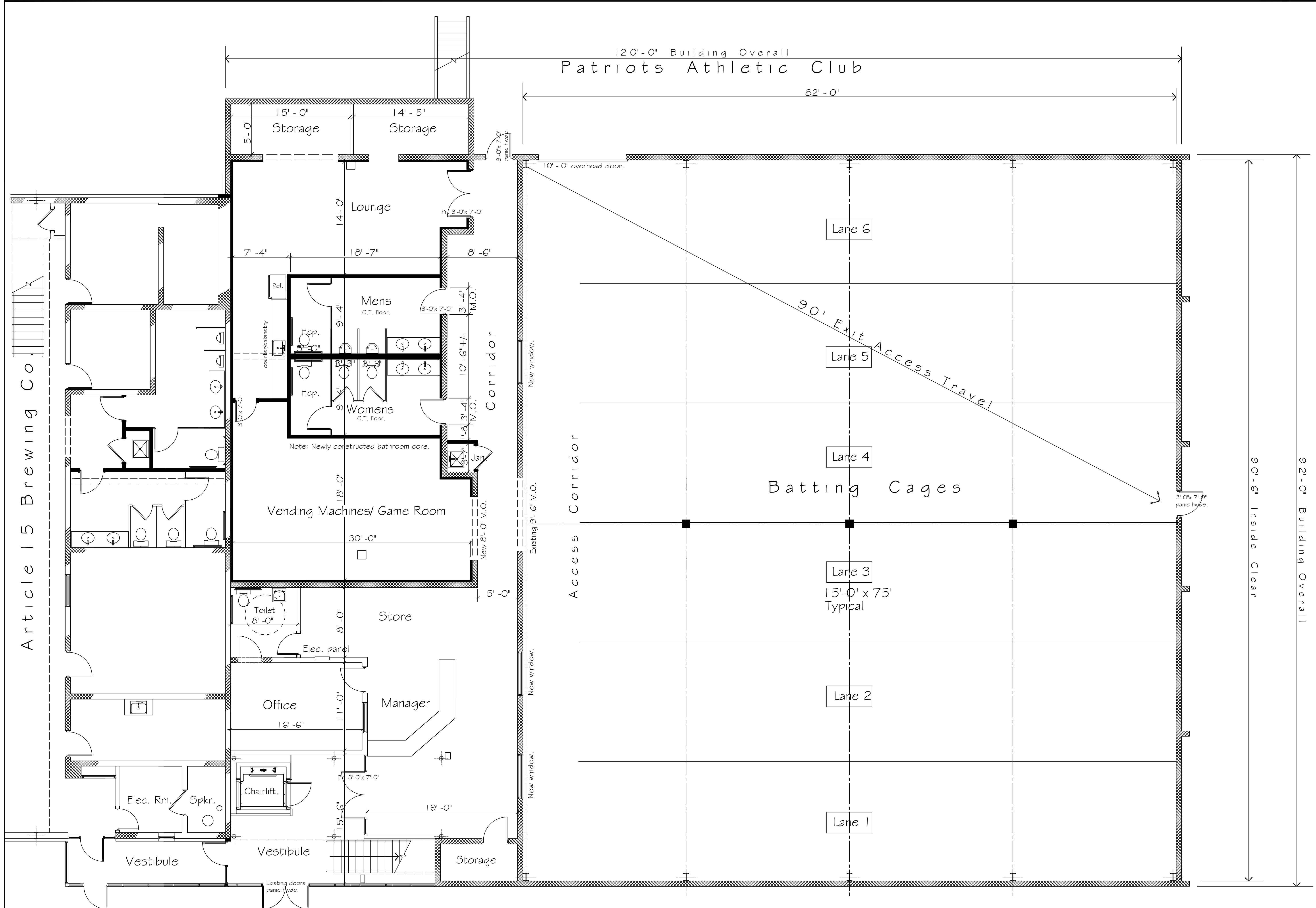
Proposed Plan @ Ground Floor 3/16" = 1'-0"
