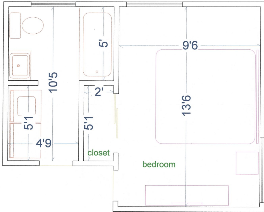
Existing Floor Plan scale 1/4" = 1'
